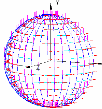
Figure 12 Cartesian Polarization Basis (LI), E_x , E_y
